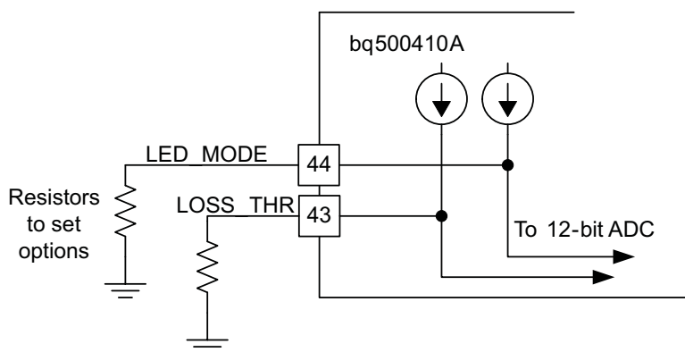
Figure 4. Option Programming
